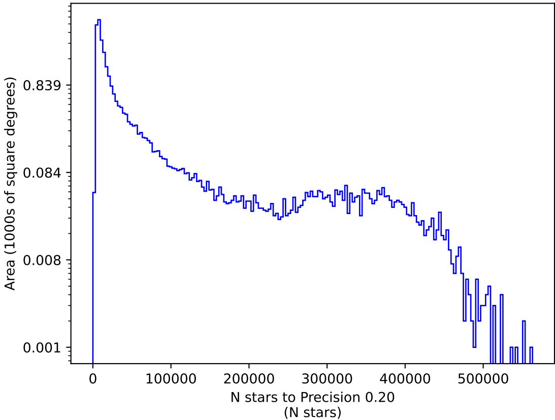
ddf_acor_sf20_lsf30_lsr50_v3.4_10yrs g: N stars to Precision 0.20
