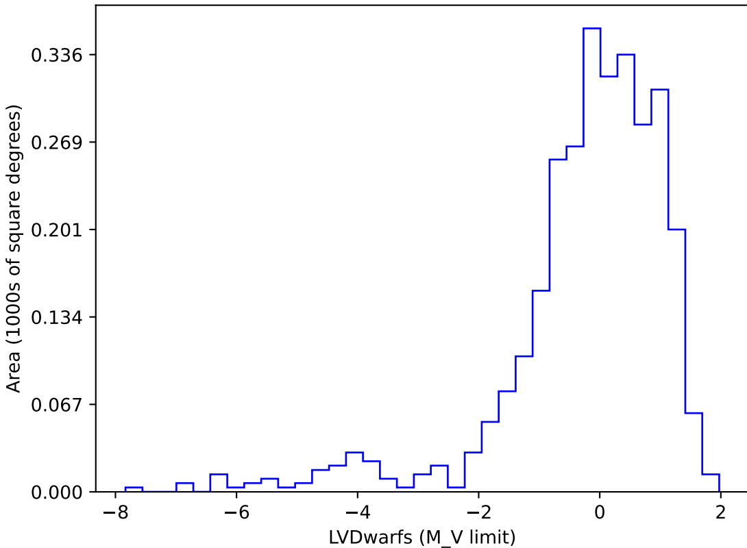
ddf_acor_sf20_lsf30_lsr50_v3.4_10yrs gi SCP: LVDwarfs
