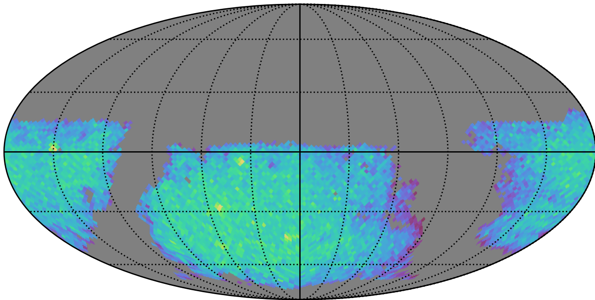
ddf_acor_sf20_lsf30_lsr50_v3.4_10yrs gi: LVDwarfs
