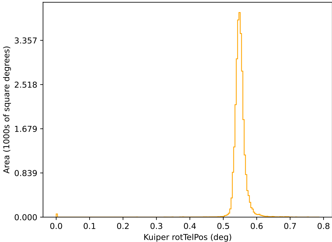
ddf_acor_sf20_lsf30_lsr50_v3.4_10yrs r: Kuiper rotTelPos
