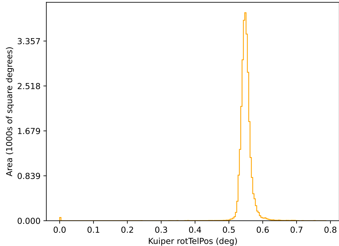
ddf_acor_sf20_lsf30_lsr50_v3.4_10yrs r: Kuiper rotTelPos
