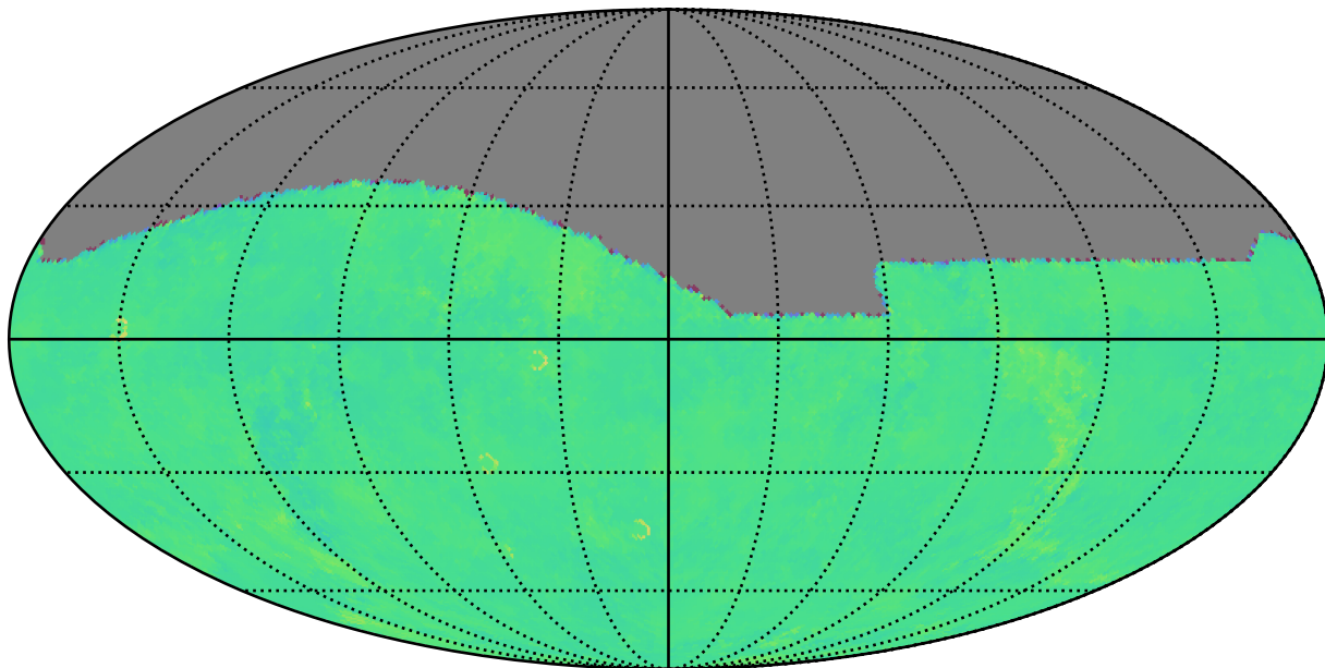
ddf_acor_sf20_lsf30_lsr50_v3.4_10yrs g: Kuiper rotTelPos
