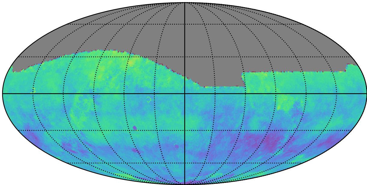
ddf_acor_sf20_lsf30_lsr50_v3.4_10yrs z: Kuiper rotSkyPos
