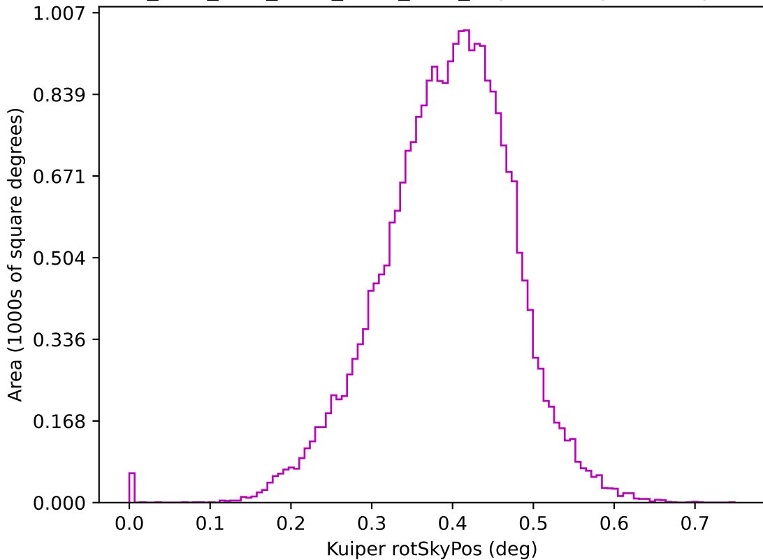
ddf_acor_sf20_lsf30_lsr50_v3.4_10yrs z: Kuiper rotSkyPos
