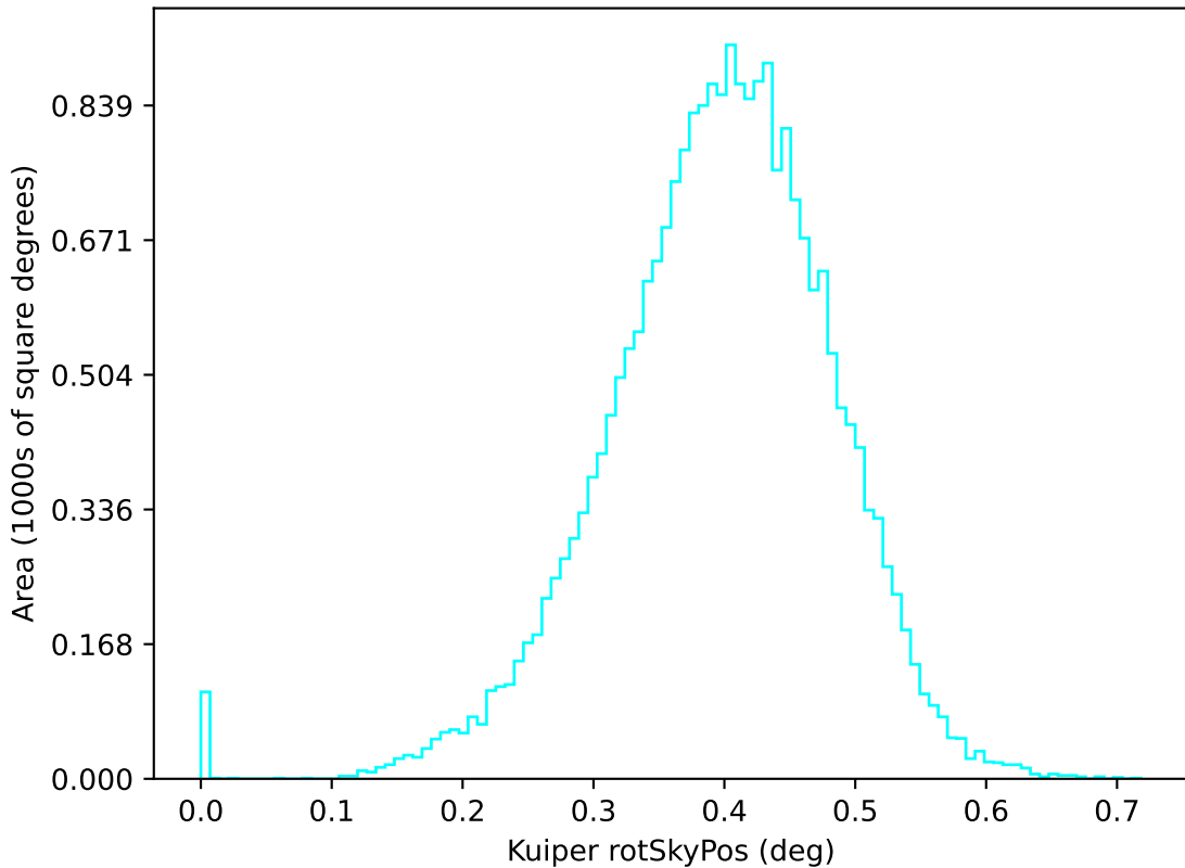
ddf_acor_sf20_lsf30_lsr50_v3.4_10yrs u: Kuiper rotSkyPos
