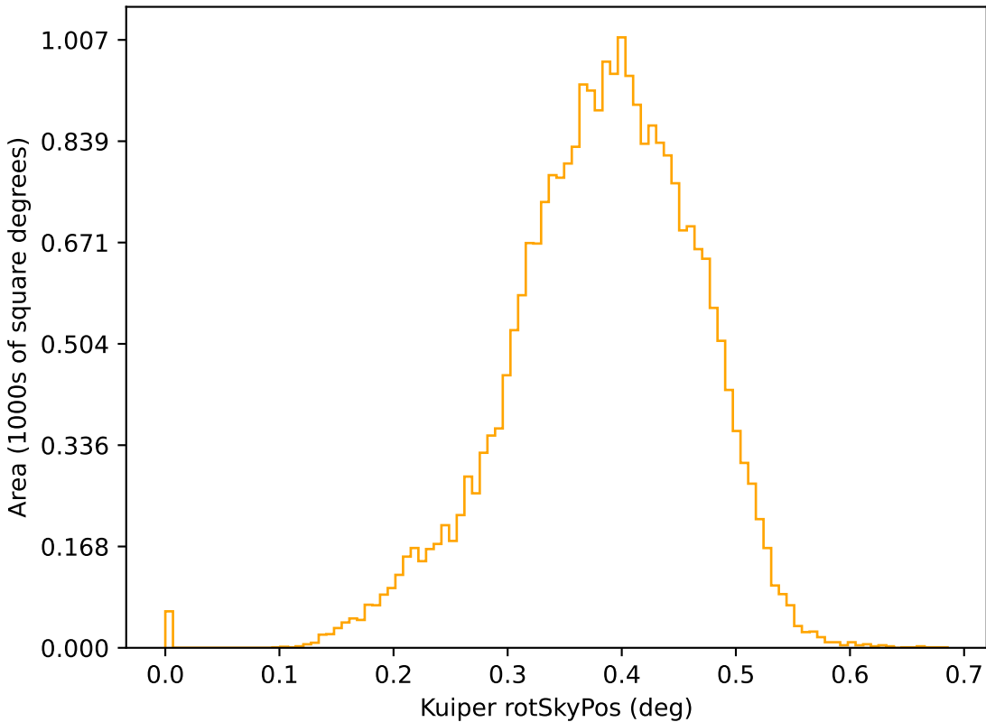
ddf_acor_sf20_lsf30_lsr50_v3.4_10yrs r: Kuiper rotSkyPos
