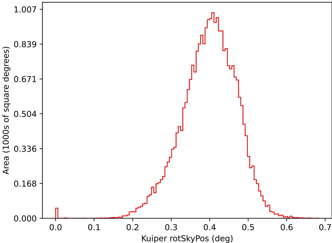
ddf_acor_sf20_ls30_lsr50_v3.4_10yrs i: Kuiper rotSkyPos
