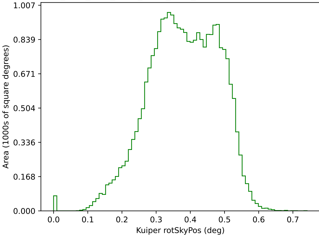
ddf_acor_sf20_lsf30_lsr50_v3.4_10yrs g: Kuiper rotSkyPos
