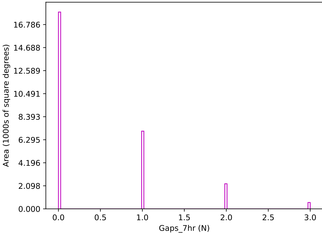
ddf_acor_sf20_lsf30_lsr50_v3.4_10yrs z band: Gaps_7hr
