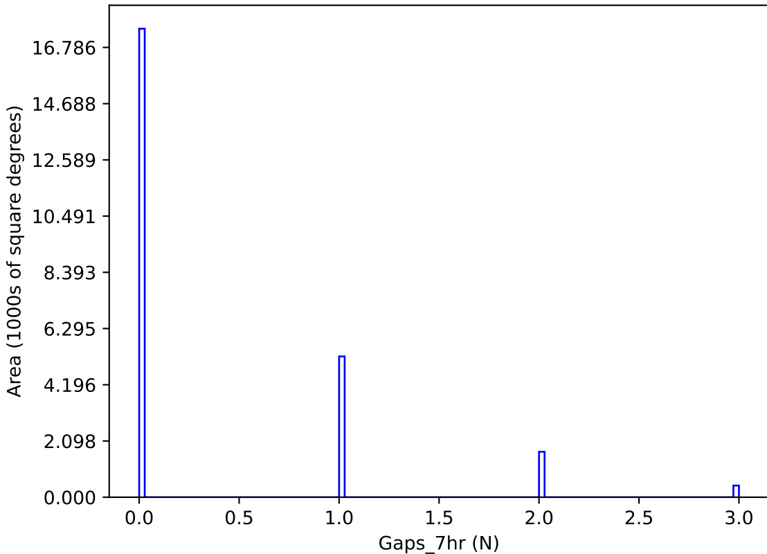
ddf_acor_sf20_ls30_lsr50_v3.4_10yrs y band: Gaps_7hr
