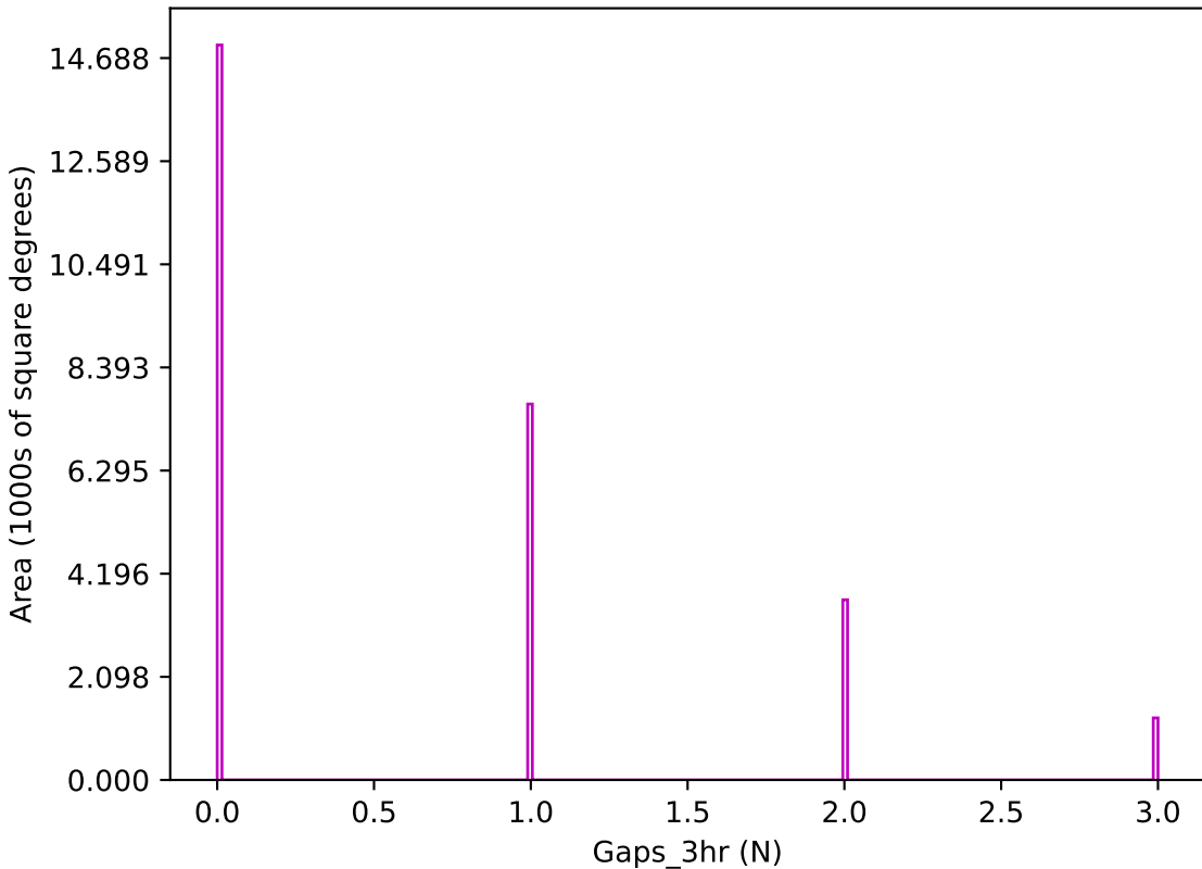
ddf_acor_sf20_ls30_lsr50_v3.4_10yrs z band: Gaps_3hr
