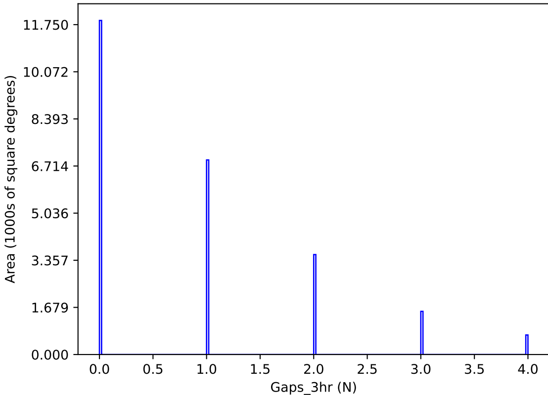
ddf_acor_sf20_lsf30_lsr50_v3.4_10yrs y band: Gaps_3hr
