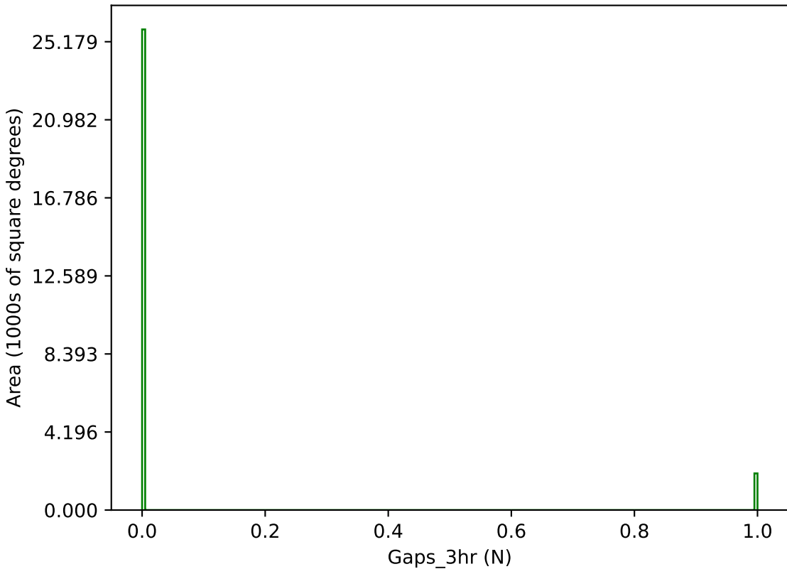
ddf_acor_sf20_lsf30_lsr50_v3.4_10yrs g band: Gaps_3hr
