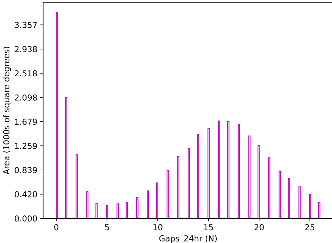
ddf_acor_sf20_lsf30_lsr50_v3.4_10yrs z band: Gaps_24hr
