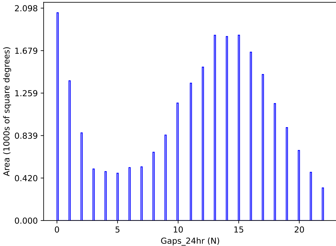
ddf_acor_sf20_lsf30_lsr50_v3.4_10yrs y band: Gaps_24hr
