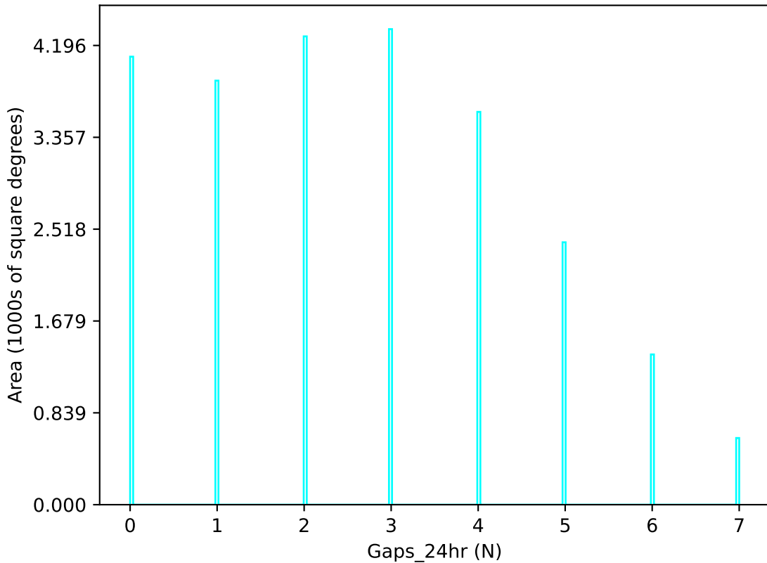
ddf_acor_sf20_lsf30_lsr50_v3.4_10yrs u band: Gaps_24hr
