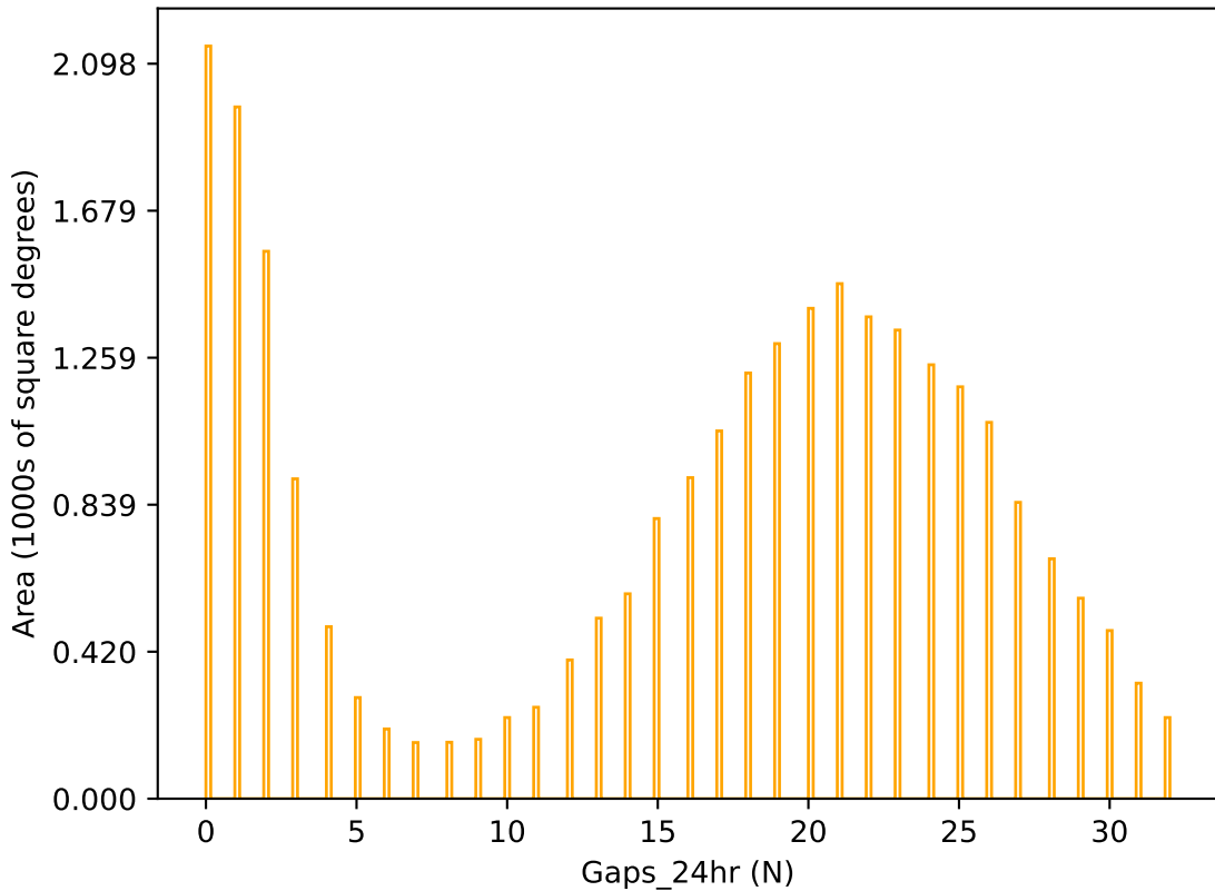
ddf_acor_sf20_lsf30_lsr50_v3.4_10yrs r band: Gaps_24hr
