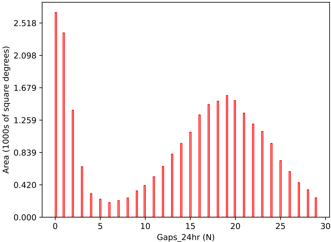
ddf_acor_sf20_lsf30_lsr50_v3.4_10yrs i band: Gaps_24hr
