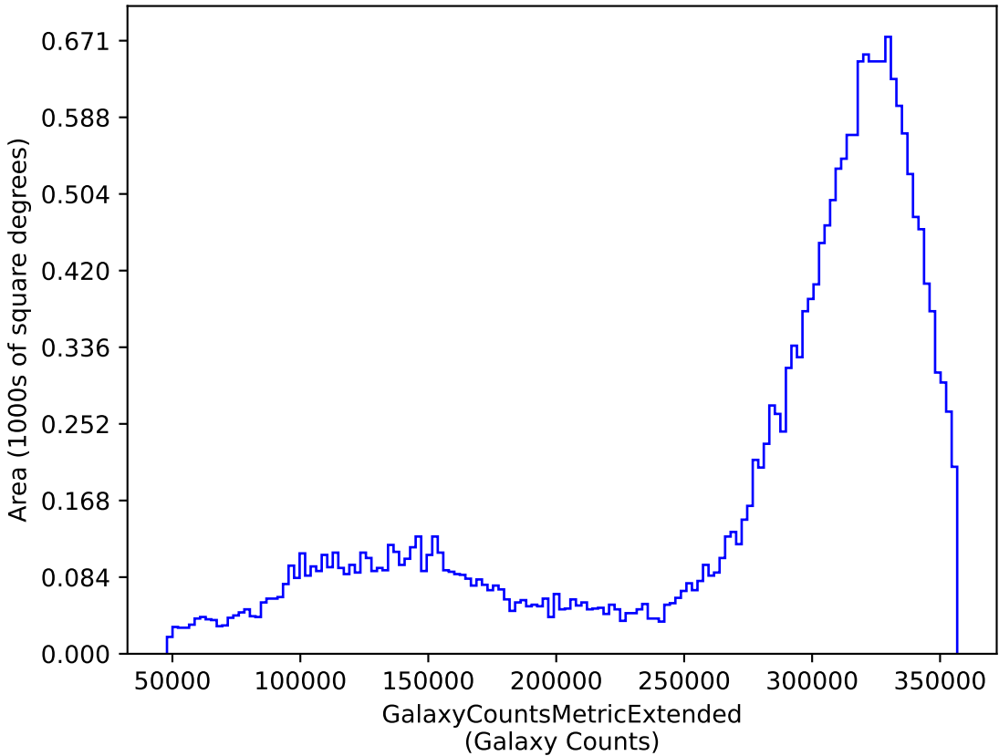
ddf_acor_sf20_lsf30_lsr50_v3.4_10yrs y: GalaxyCountsMetricExtended
