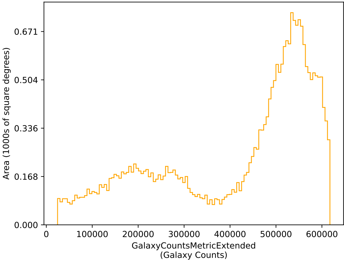
ddf_acor_sf20_lsf30_lsr50_v3.4_10yrs r: GalaxyCountsMetricExtended
