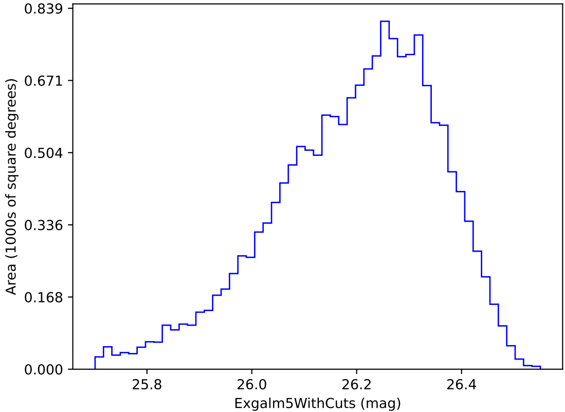
ddf_acor_sf20_lsf30_lsr50_v3.4_10yrs i band non-DD year 7: ExgalM5WithCuts
