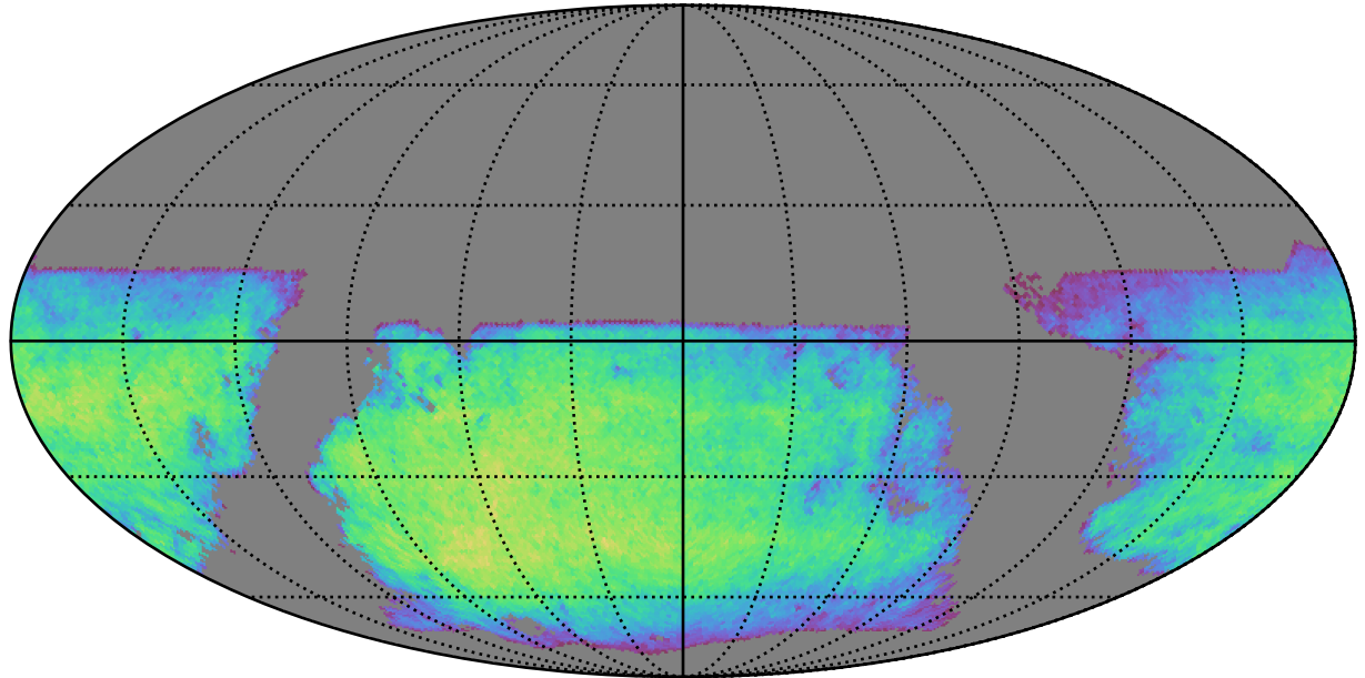
ddf_acor_sf20_lsf30_lsr50_v3.4_10yrs i band non-DD year 10: ExgalM5WithCuts
