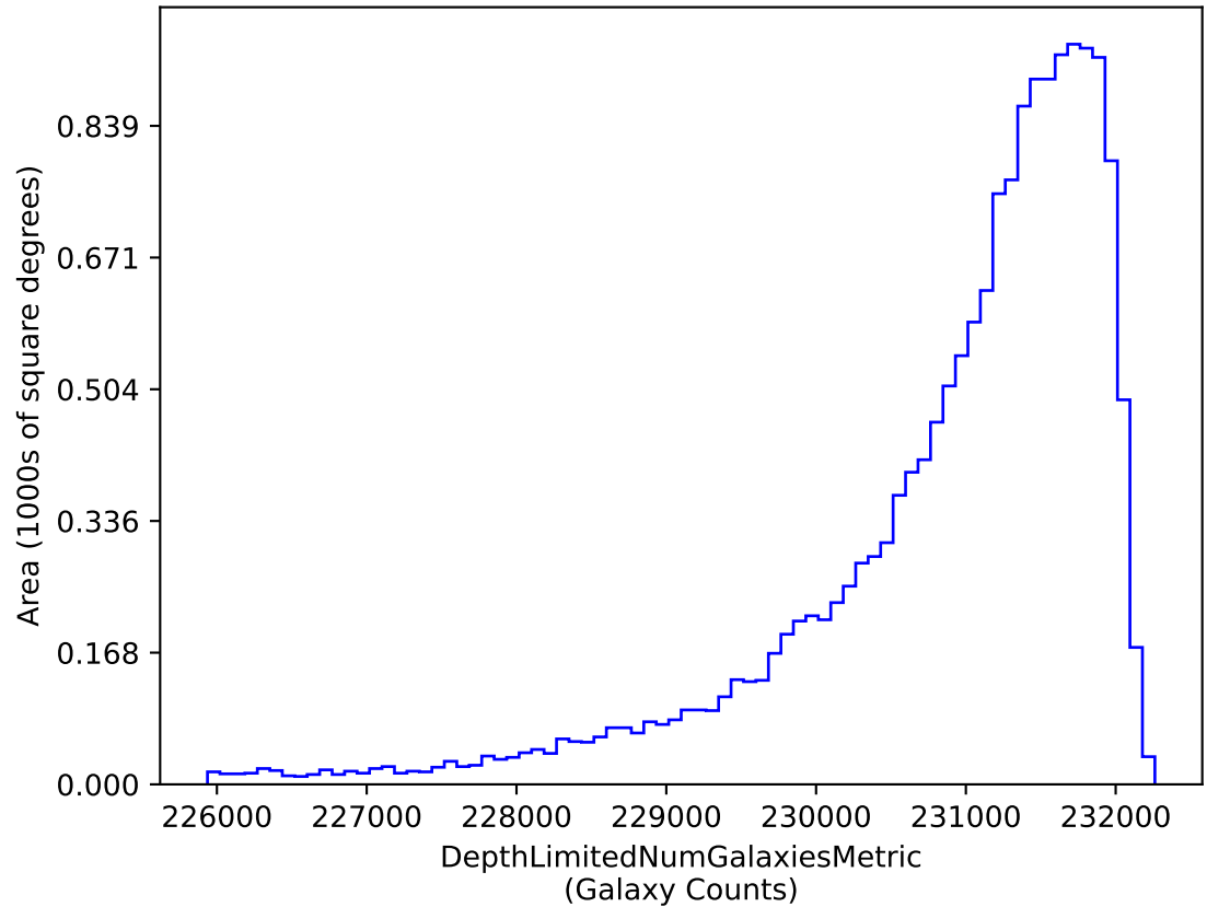
ddf_acor_sf20_lsf30_lsr50_v3.4_10yrs i band galaxies non-DD: DepthLimitedNumGalaxiesMetric
