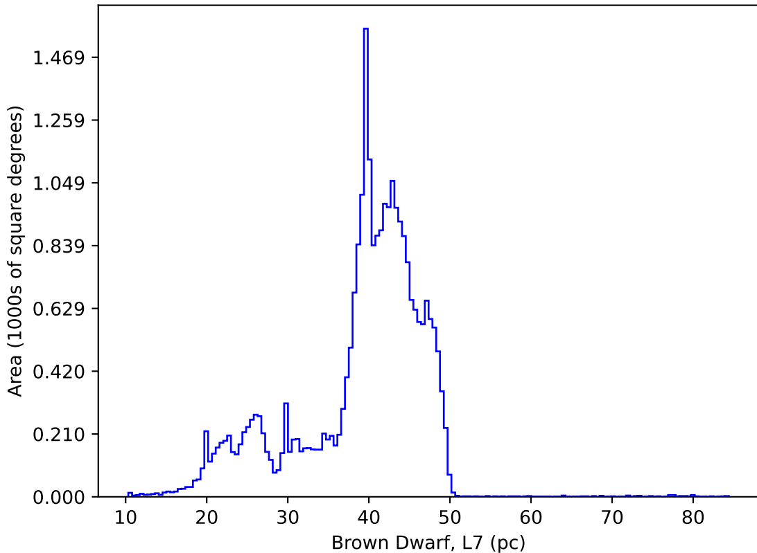
ddf_acor_sf20_lsf30_lsr50_v3.4_10yrs : Brown Dwarf, L7
