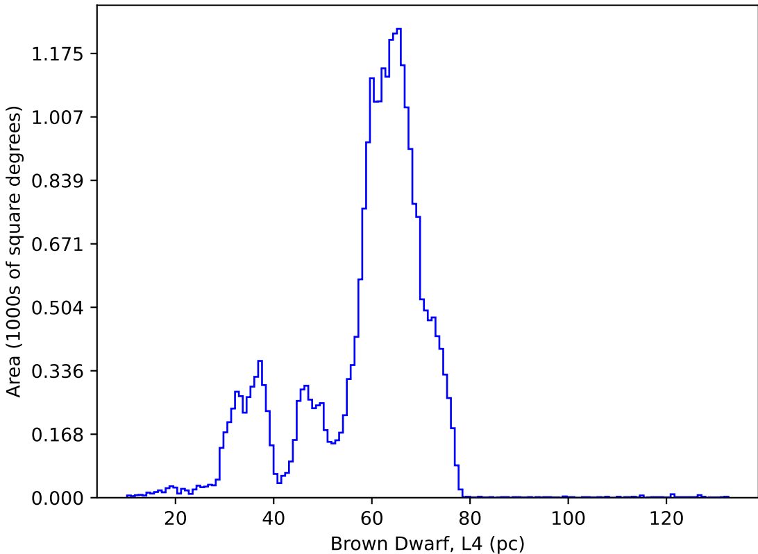
ddf_acor_sf20_lsf30_lsr50_v3.4_10yrs : Brown Dwarf, L4
