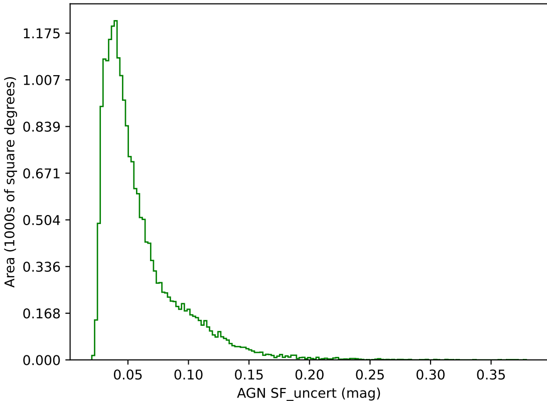
ddf_acor_sf20_lsf30_lsr50_v3.4_10yrs g band: AGN SF_uncert
