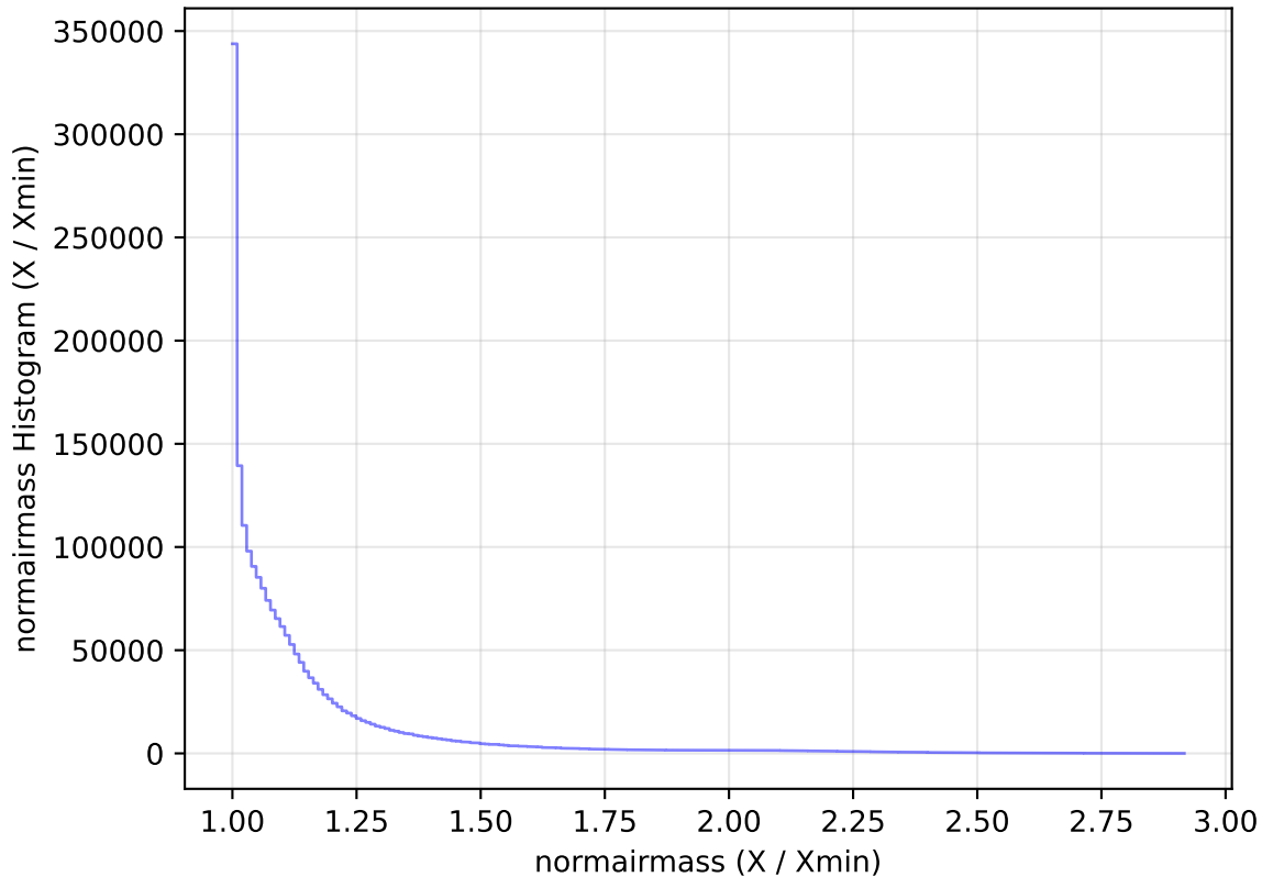
ddf_acor_sf20_lsf30_lsr50_v3.4_10yrs WFD all bands: normairmass Histogram
