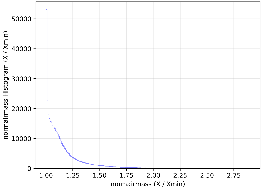
ddf_acor_sf20_lsf30_lsr50_v3.4_10yrs All sky y band: normairmass Histogram
