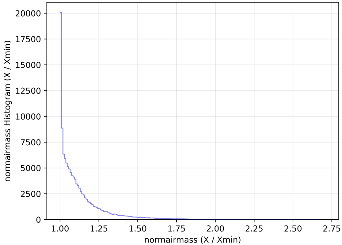
ddf_acor_sf20_lsf30_lsr50_v3.4_10yrs All sky u band: normairmass Histogram
