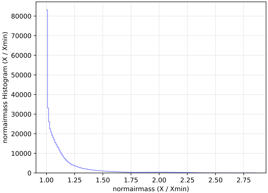
ddf_acor_sf20_lsf30_lsr50_v3.4_10yrs All sky r band: normairmass Histogram
