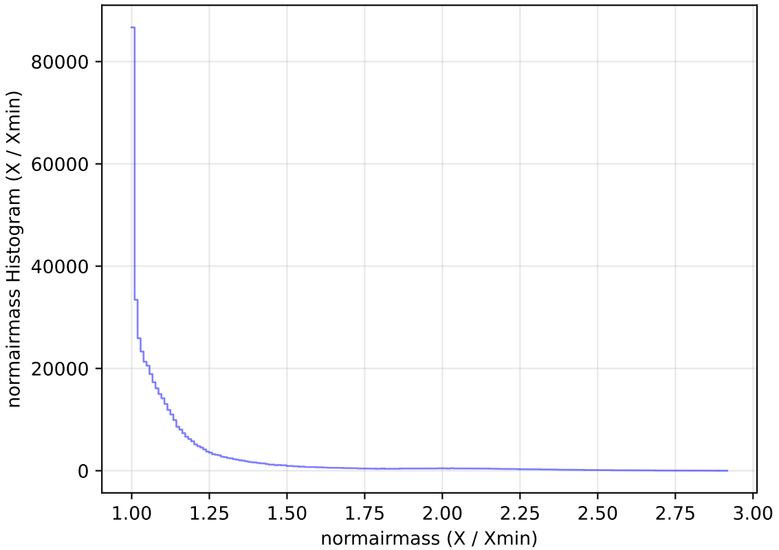
ddf_acor_sf20_lsf30_lsr50_v3.4_10yrs All sky i band: normairmass Histogram
