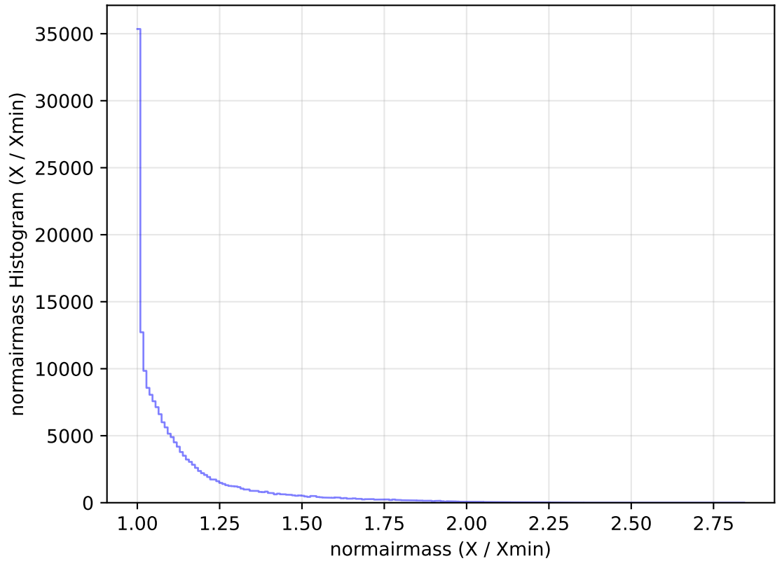
ddf_acor_sf20_lsf30_lsr50_v3.4_10yrs All sky g band: normairmass Histogram
