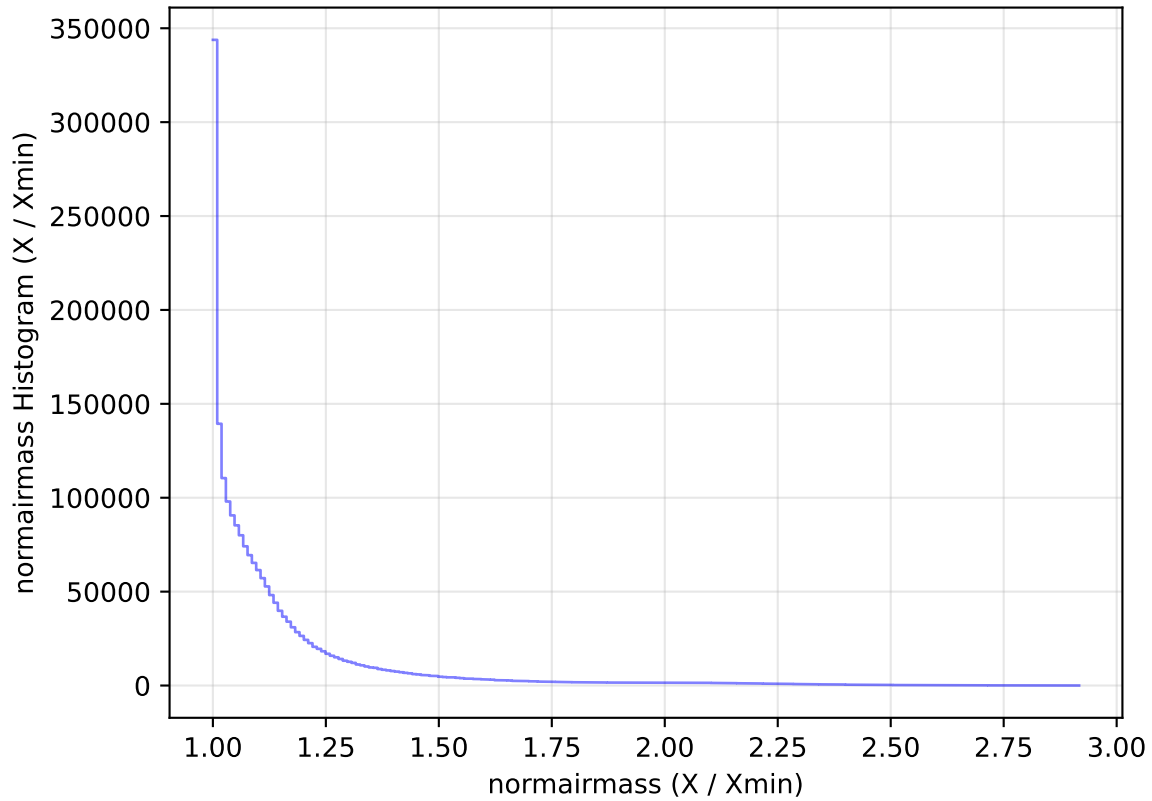
ddf_acor_sf20_lsf30_lsr50_v3.4_10yrs All sky all bands: normairmass Histogram
