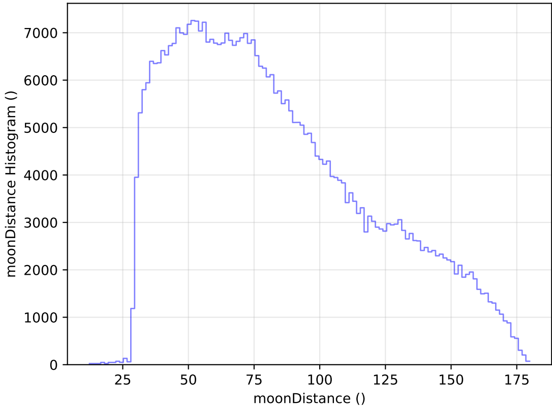
ddf_acor_sf20_lsf30_lsr50_v3.4_10yrs WFD z band: moonDistance Histogram
