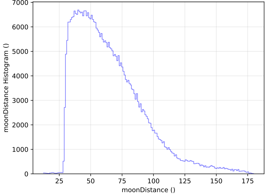
ddf_acor_sf20_Isf30_Isr50_v3.4_10yrs WFD y band: moonDistance Histogram
