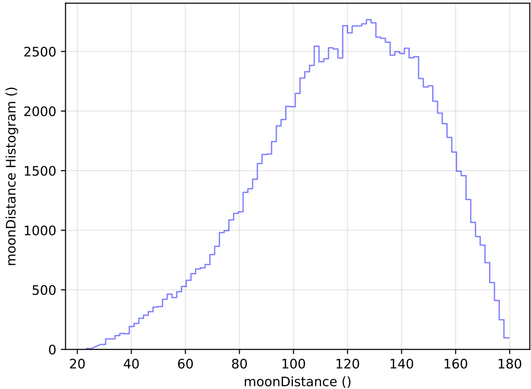
ddf_acor_sf20_lsf30_lsr50_v3.4_10yrs WFD u band: moonDistance Histogram
