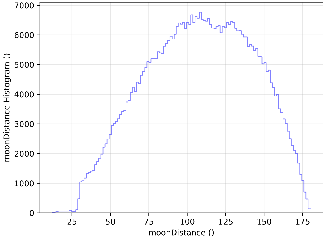
ddf_acor_sf20_lsf30_lsr50_v3.4_10yrs WFD r band: moonDistance Histogram
