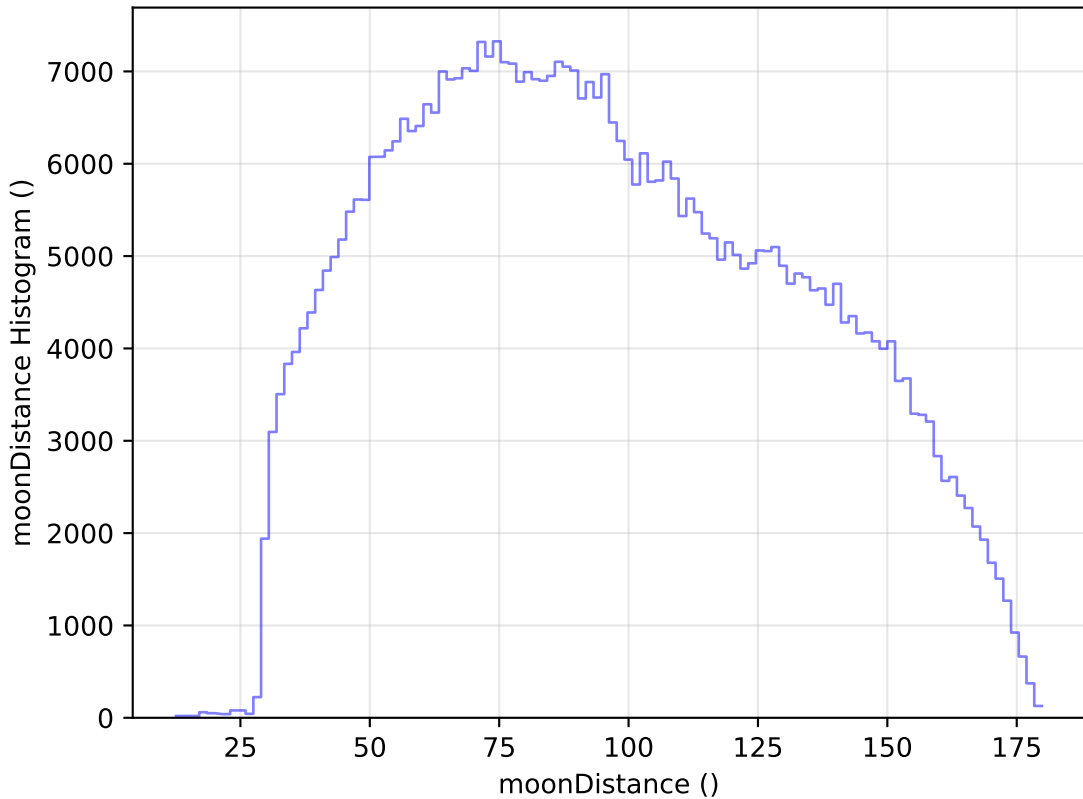
ddf_acor_sf20_lsf30_lsr50_v3.4_10yrs WFD i band: moonDistance Histogram
