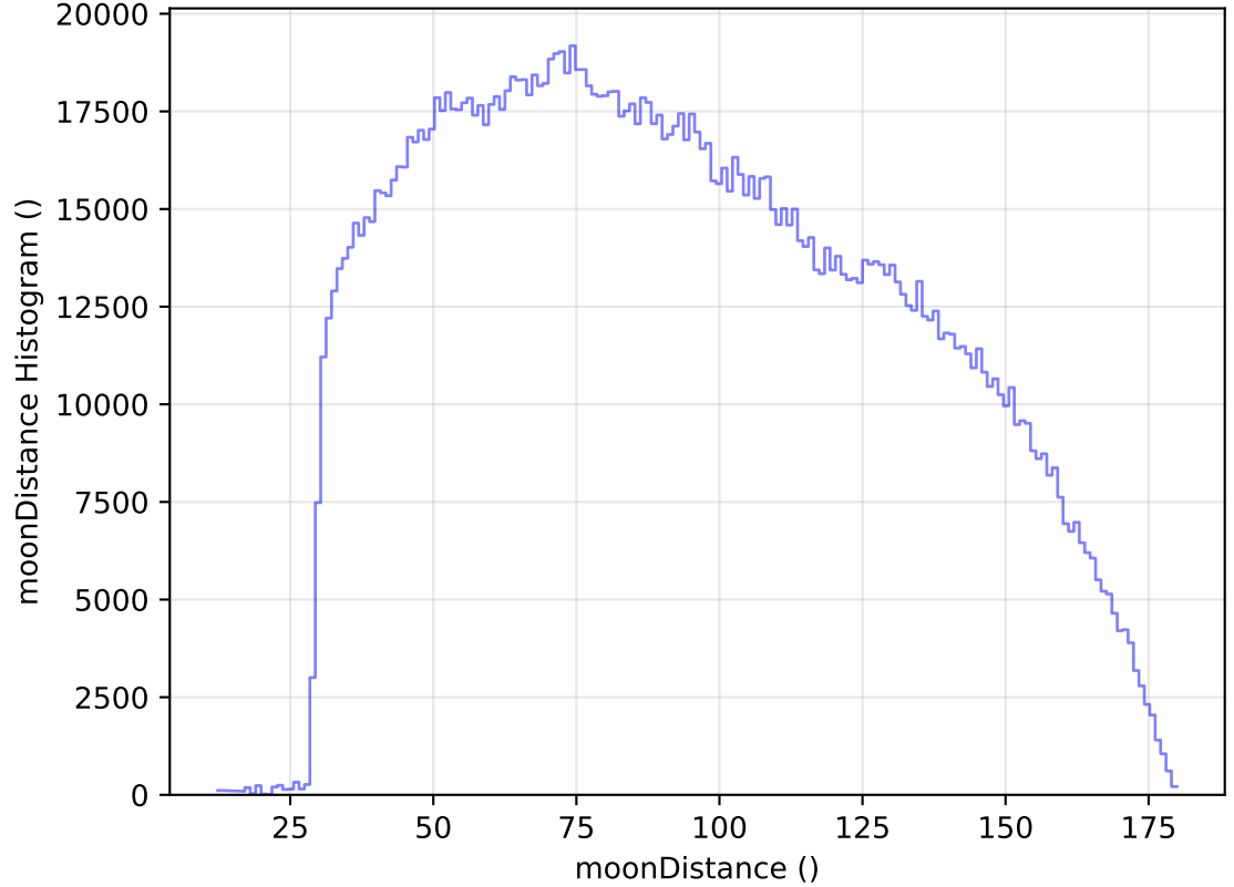
ddf_acor_sf20_lsf30_lsr50_v3.4_10yrs WFD all bands: moonDistance Histogram
