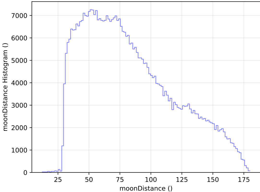
ddf_acor_sf20_lsf30_lsr50_v3.4_10yrs All sky z band: moonDistance Histogram
