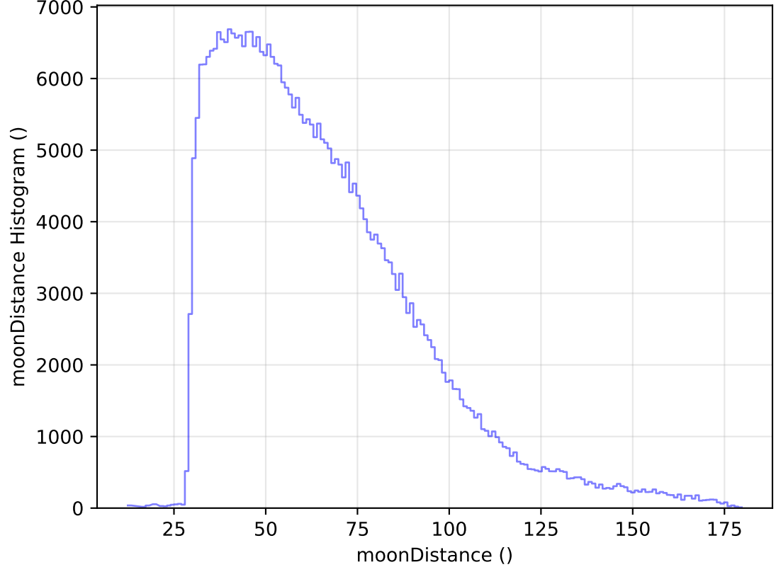
ddf_acor_sf20_lsf30_lsr50_v3.4_10yrs All sky y band: moonDistance Histogram
