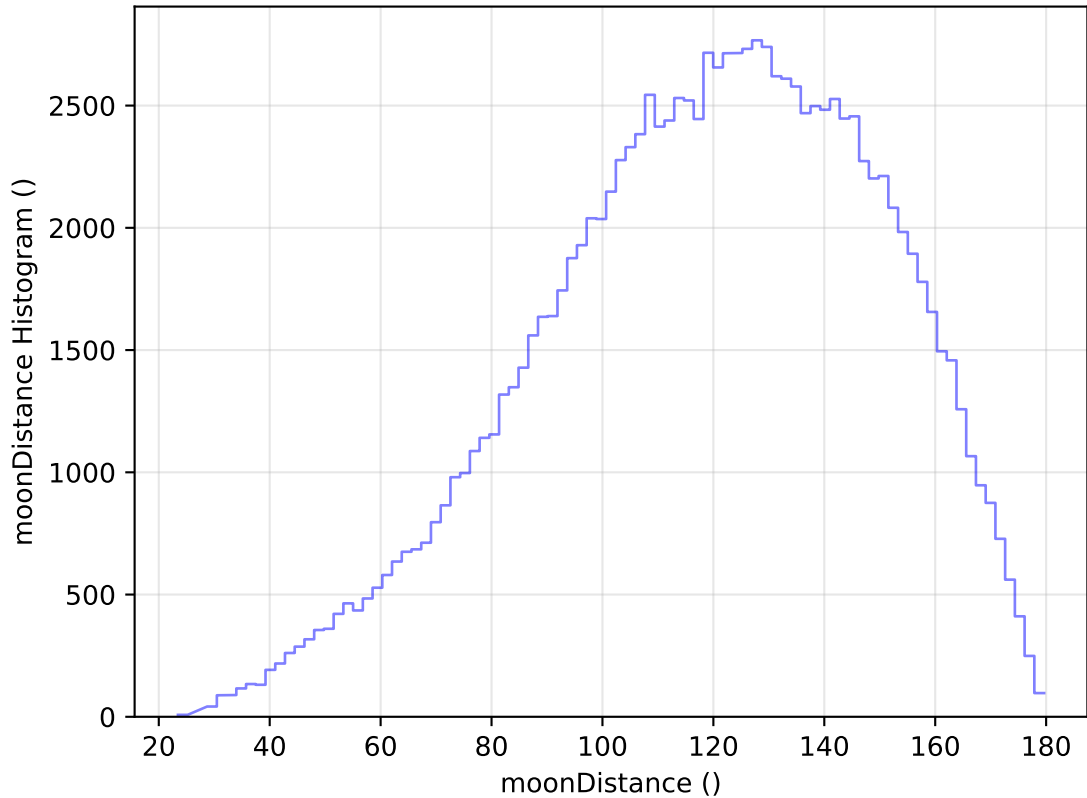
ddf_acor_sf20_lsf30_lsr50_v3.4_10yrs All sky u band: moonDistance Histogram
