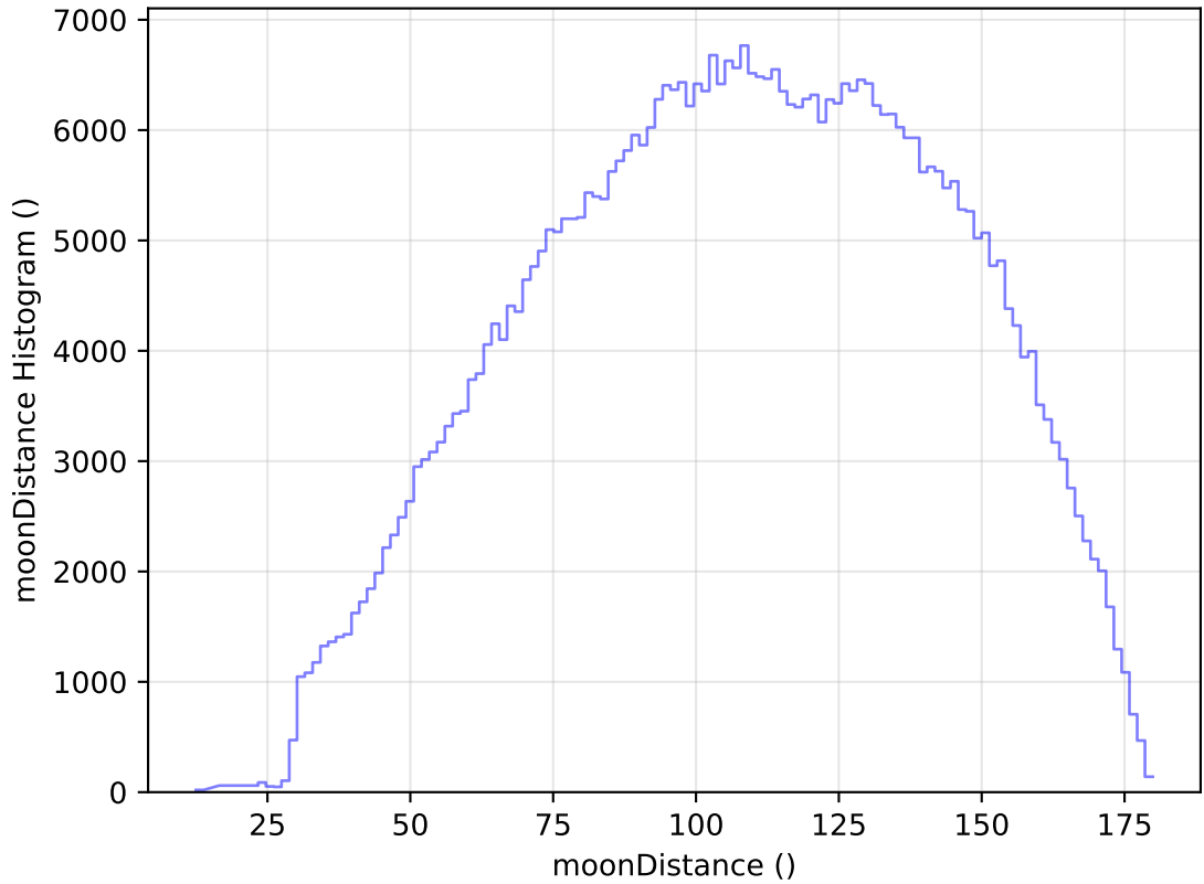
ddf_acor_sf20_lsf30_lsr50_v3.4_10yrs All sky r band: moonDistance Histogram
