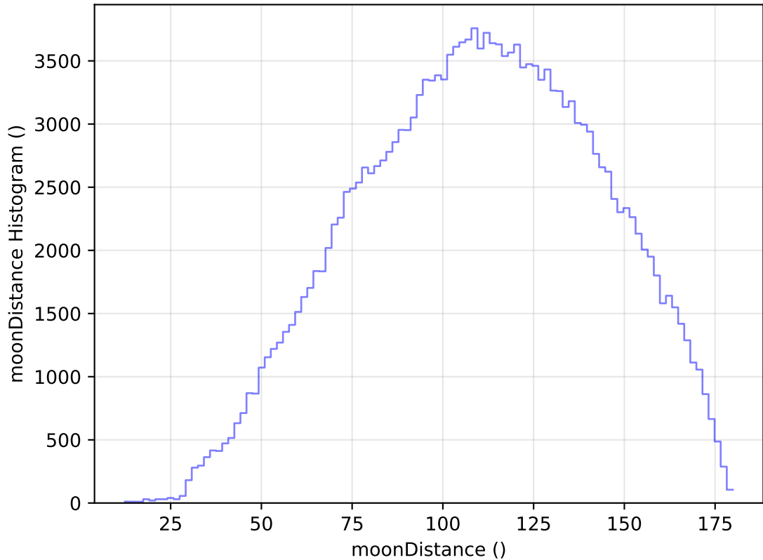
ddf_acor_sf20_lsf30_lsr50_v3.4_10yrs All sky g band: moonDistance Histogram
