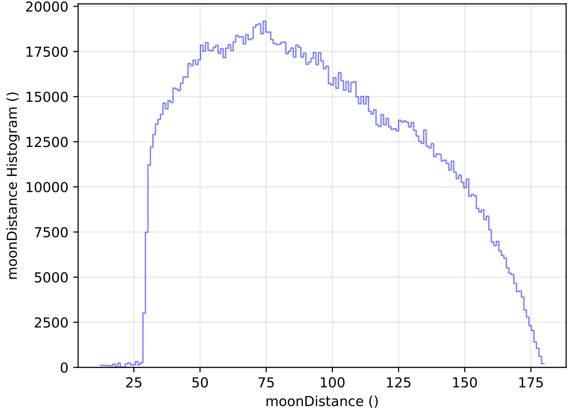
ddf_acor_sf20_lsf30_lsr50_v3.4_10yrs All sky all bands: moonDistance Histogram
