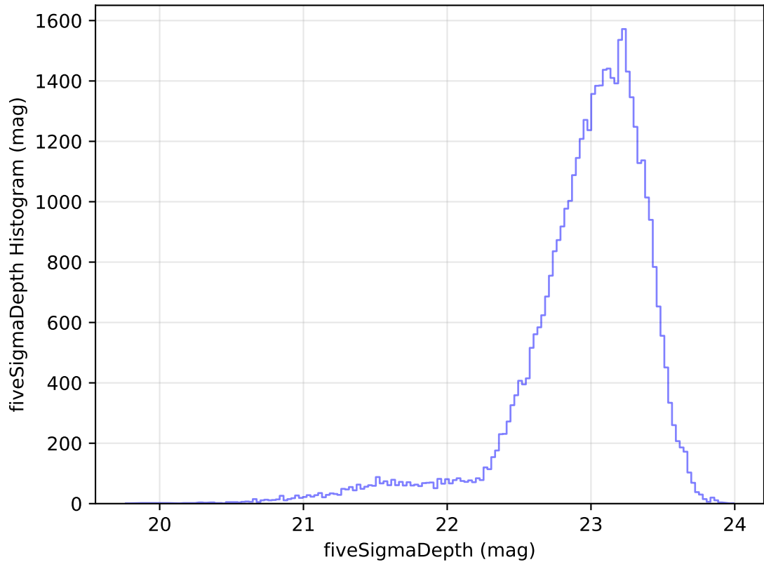
ddf_acor_sf20_lsf30_lsr50_v3.4_10yrs Yr 1 z band: fiveSigmaDepth Histogram
