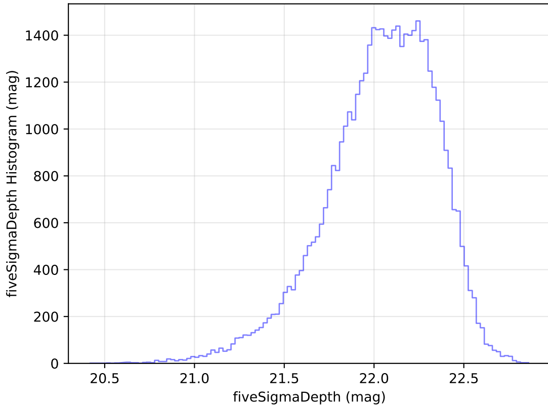
ddf_acor_sf20_lsf30_lsr50_v3.4_10yrs Yr 1 y band: fiveSigmaDepth Histogram
